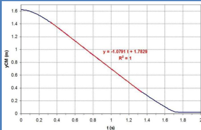
Settling of a solid particle in a viscous fluid: Velocity contours (left); Evolution in time of the y-coordinate of the solid center of mass and linear regression (right)
